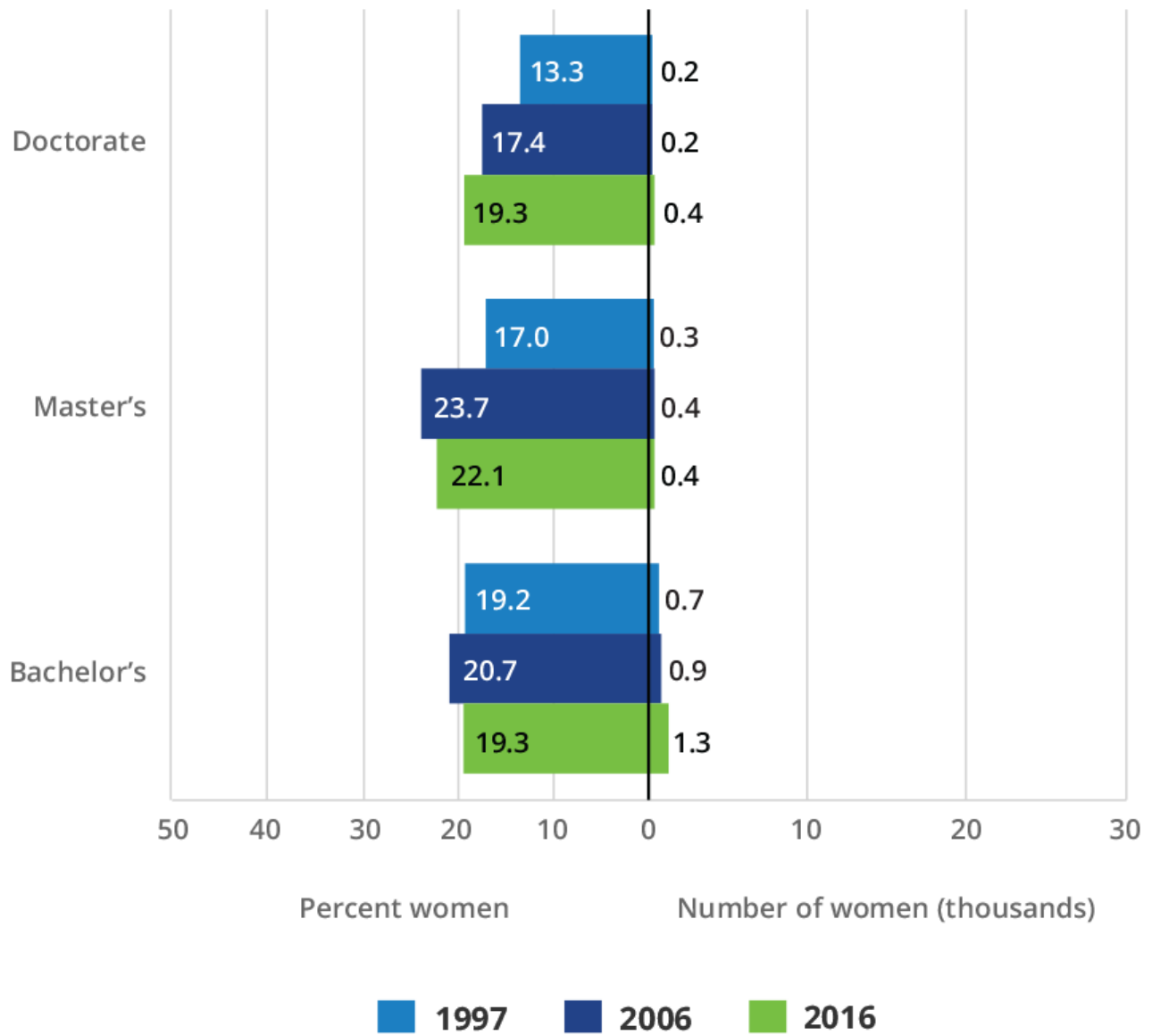
FIGURE 2-F Degrees awarded to women: Physics, 1997, 2006, 2016
