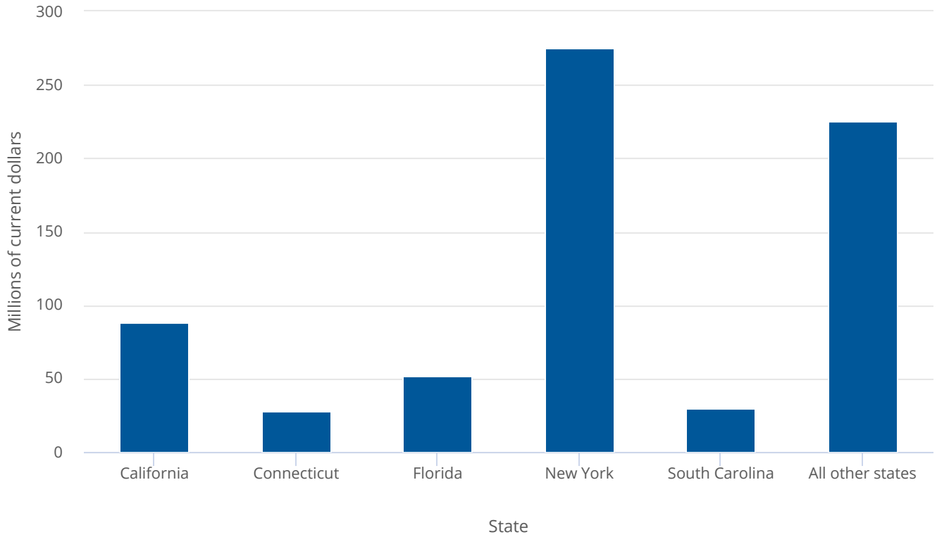
State government expenditures for R&D for intramural performers, by state and source of funds: FY 2022
